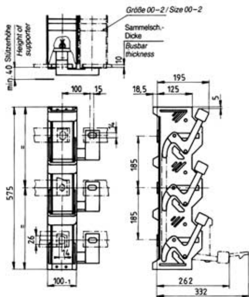
NH-Sicherungs-Koppelleiste Gr. 2: 400 A NH fuse-switch, vertical design, size 2: 400 A with coupling system
